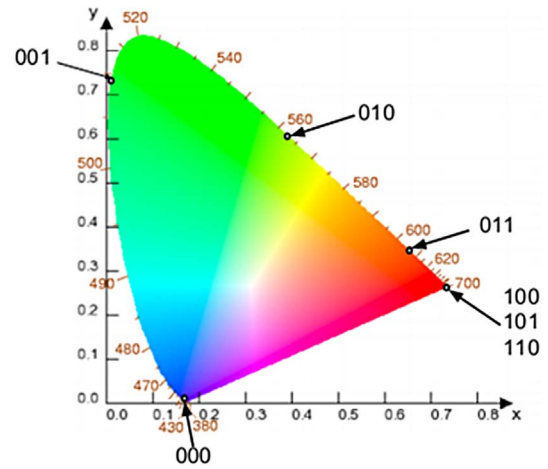
Fig. 17. Chromaticity diagram [62].
